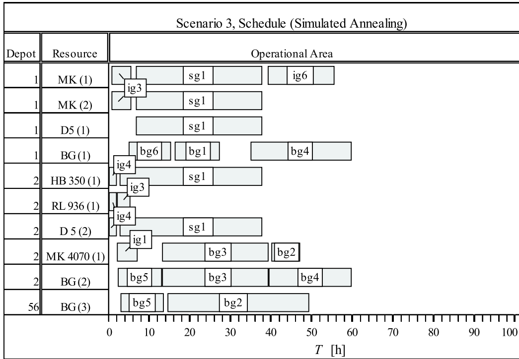
Fig. 6. Example for a calculated schedule (Simulated Annealing).
