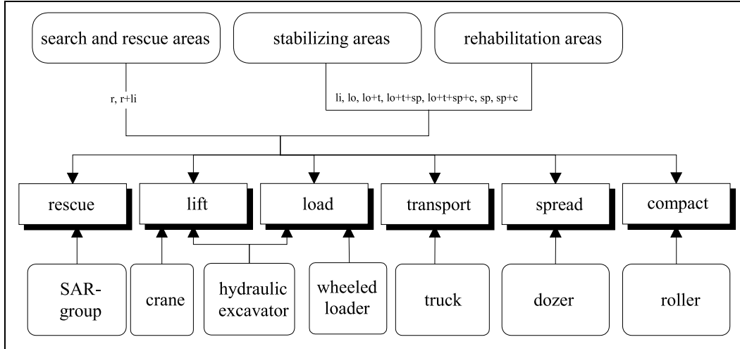
Fig. 2. Elementary work classes and the corresponding resources.
