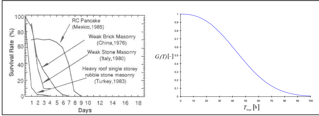
Fig. 3. Real and estimated survival rate (left picture taken from [4]).
