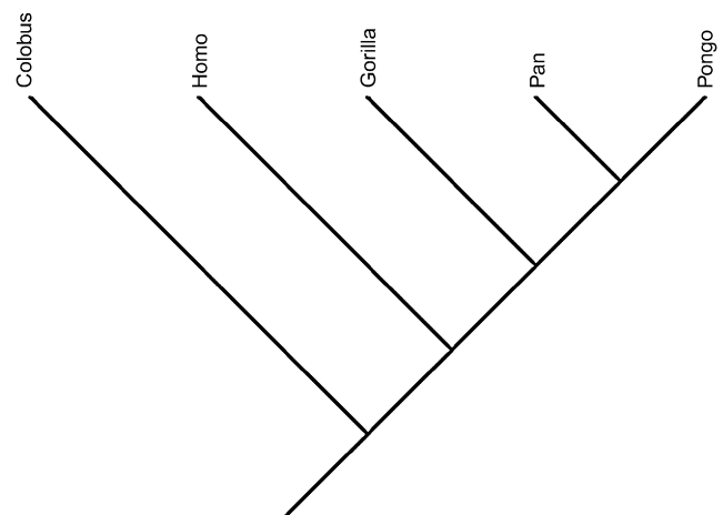
Fig. 2. Relationships suggested by the non-phenotypically-plastic measurements.
