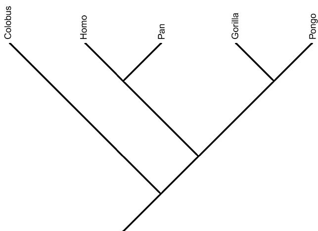
Fig. 4. Relationships suggested by the moderate-to-high-strain characters.
