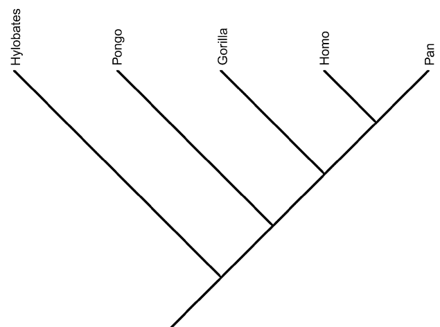
Fig. 1. Hominoid molecular relationships.
