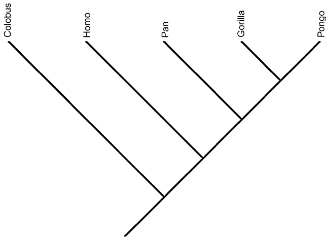
Fig. 3. Relationships suggested by the low-to-moderate-strain characters.
