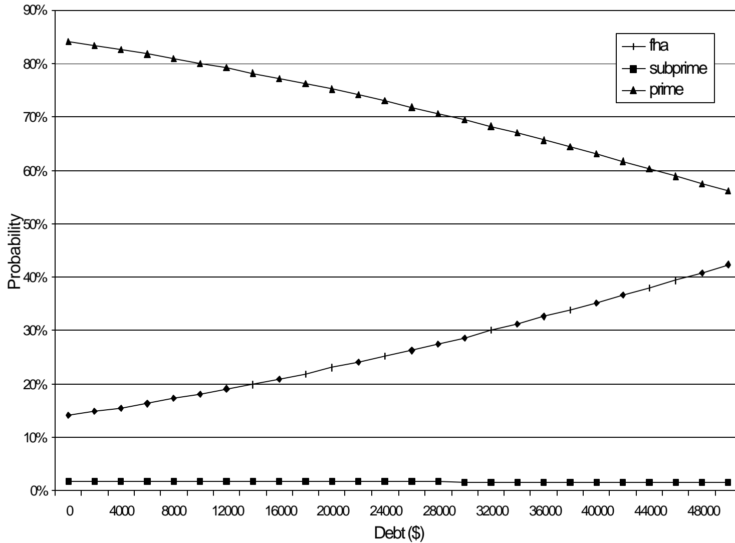
Figure 3: Mortgage Choice and Non-Real Estate Debt
