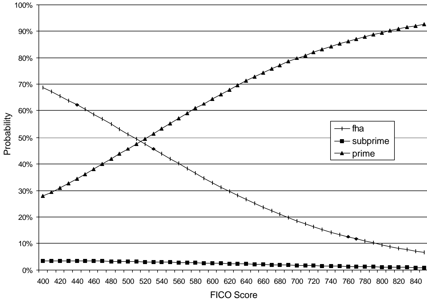
Figure 4: Mortgage Choice and FICO Scores
