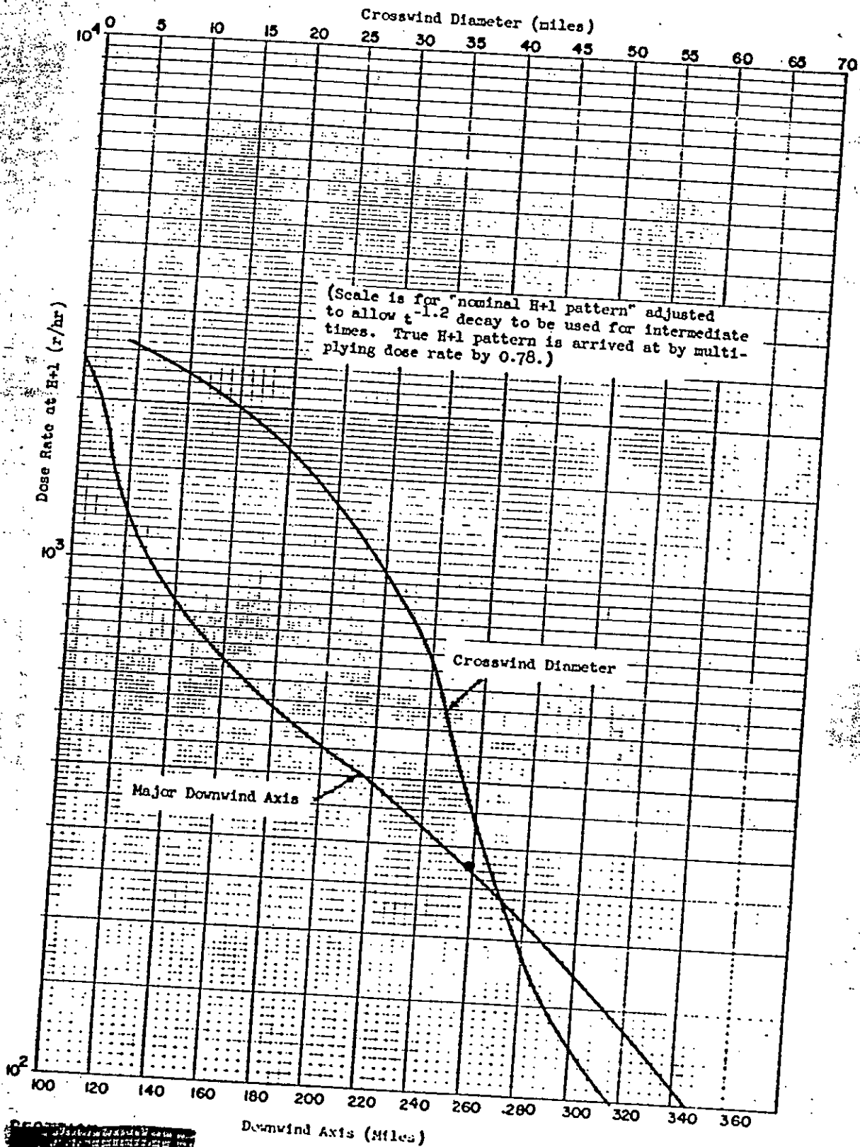
Fig. 9 DOWNWIND AND CROSSWIND AXES OF DOWNWIND PATTERN
