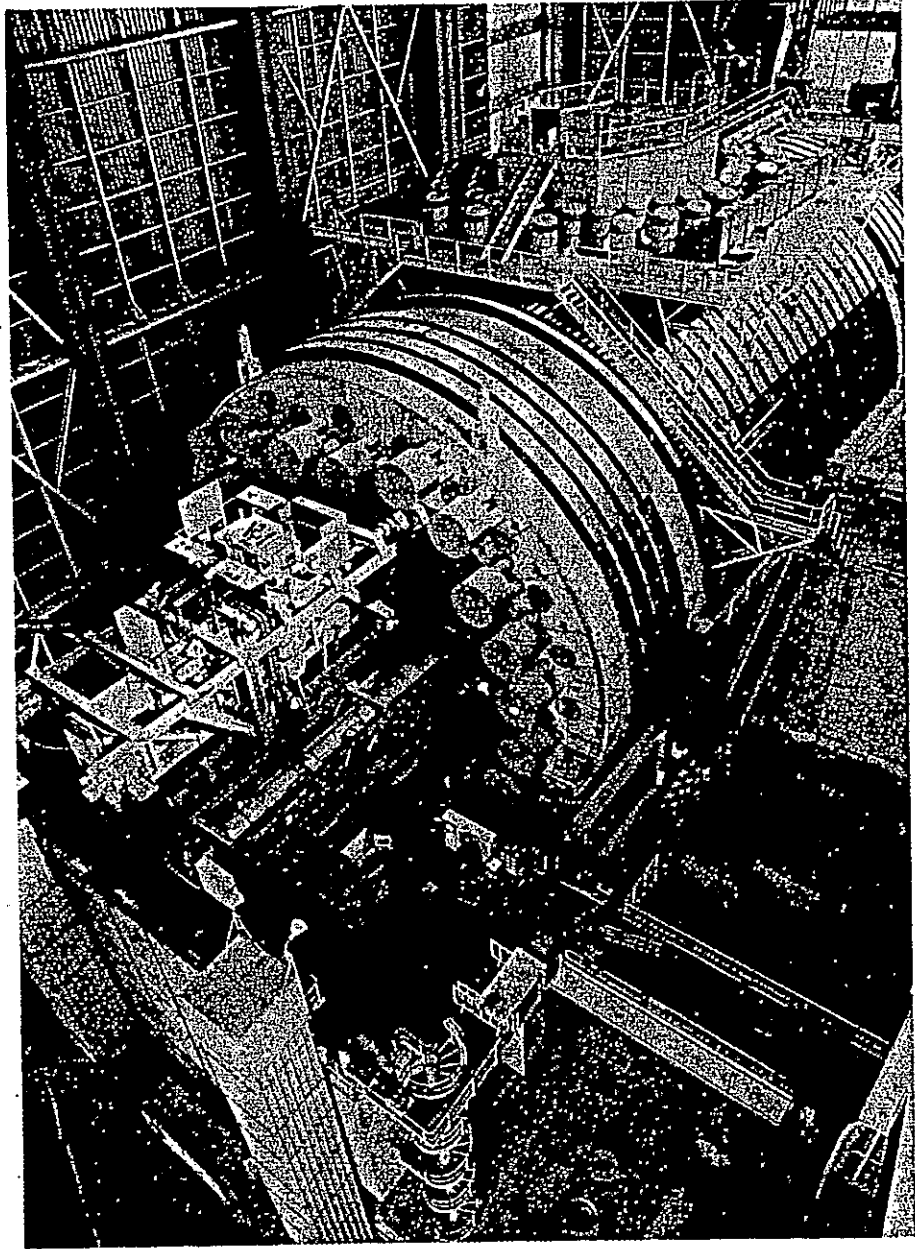
Figure 4. Shell of the G2 Reactor
